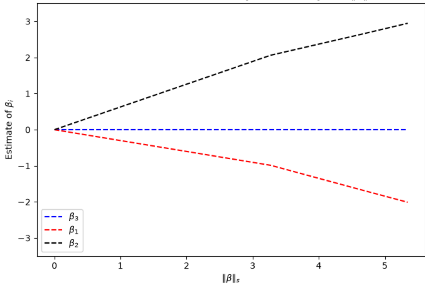
Solution Paths of L^s -Linear Regularization against \|\beta\|_s
