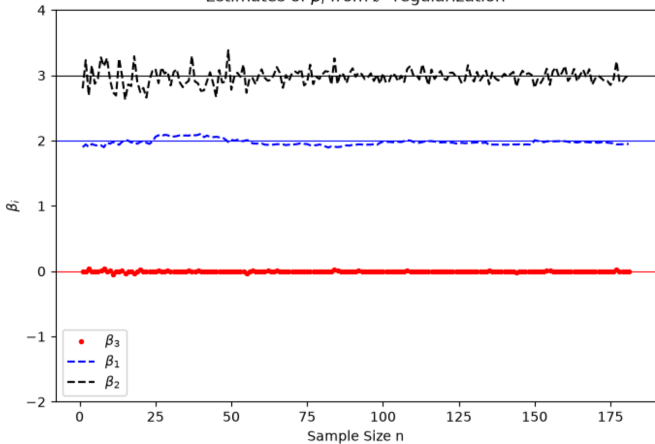
Estimates of \beta_i from \ell^s -regularization
