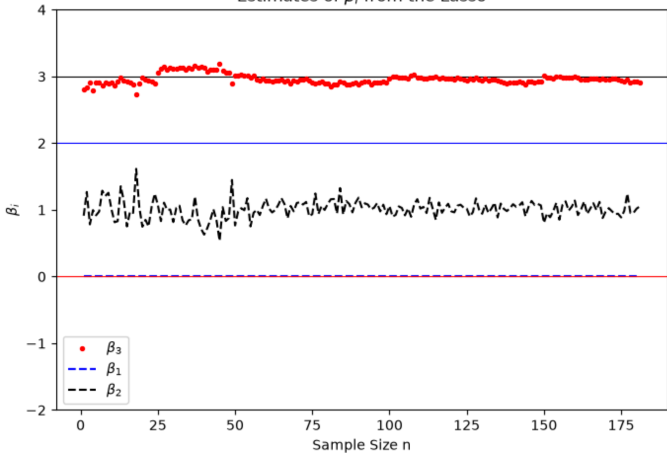
Estimates of \beta_i from the Lasso
