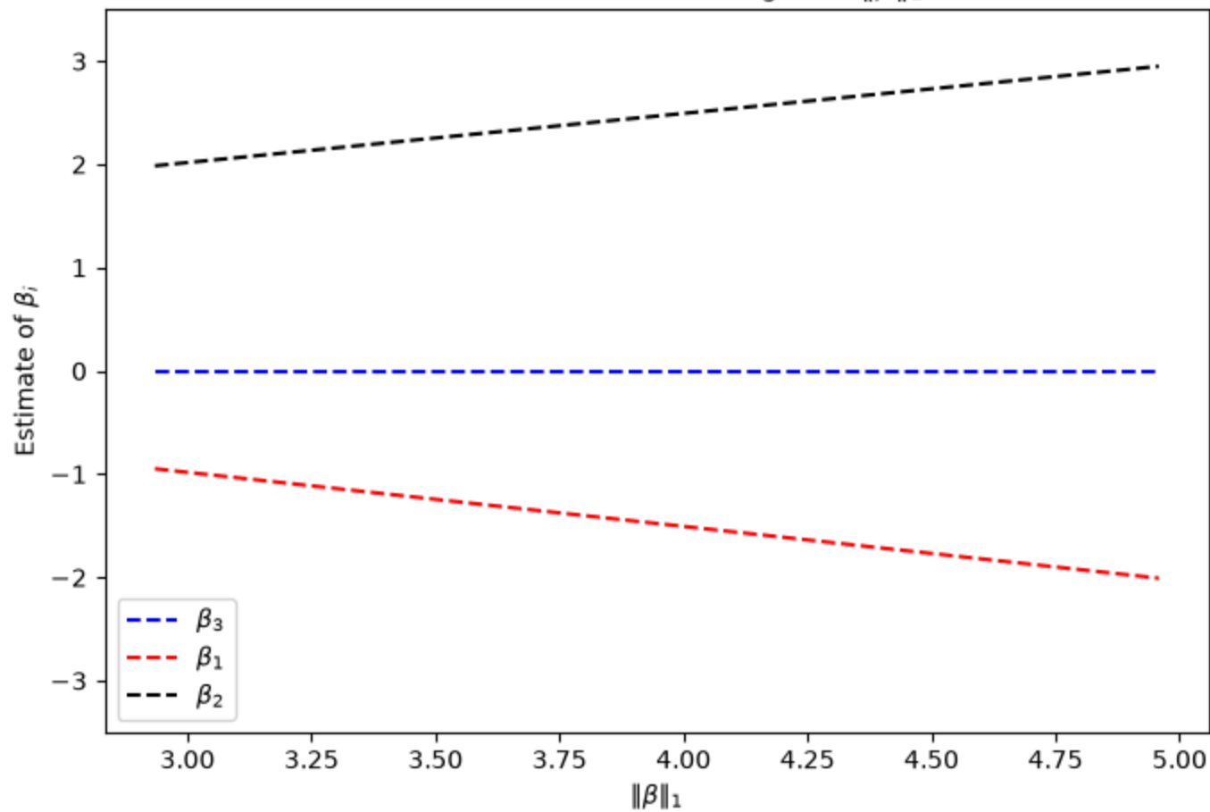
Solution Paths of Lasso against \|\beta\|_1
